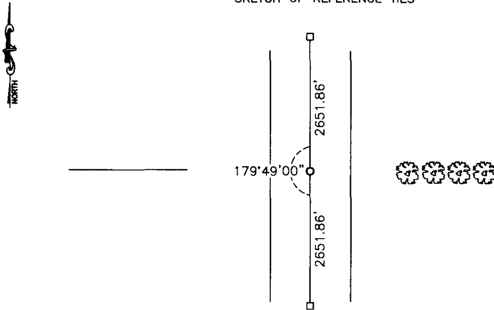
SKETCH OF REFERENCE TIES
