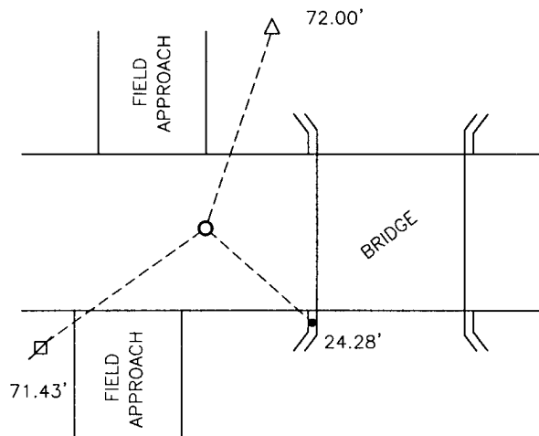
SKETCH OF REFERENCE TIES
